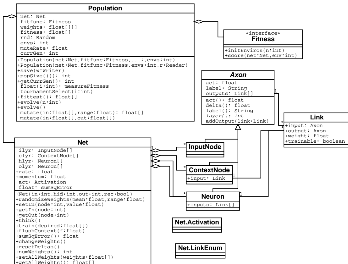
Figure 3.2: UML class diagram of neurotic package (some fields and methods are omitted for clarity).
